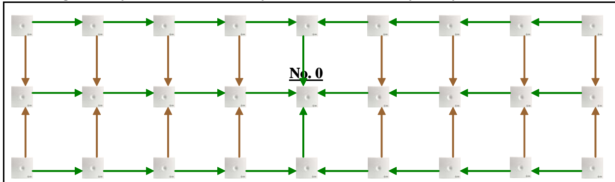
Figure 3 Synchronization Chain Layout without Alternative Sync Ways
